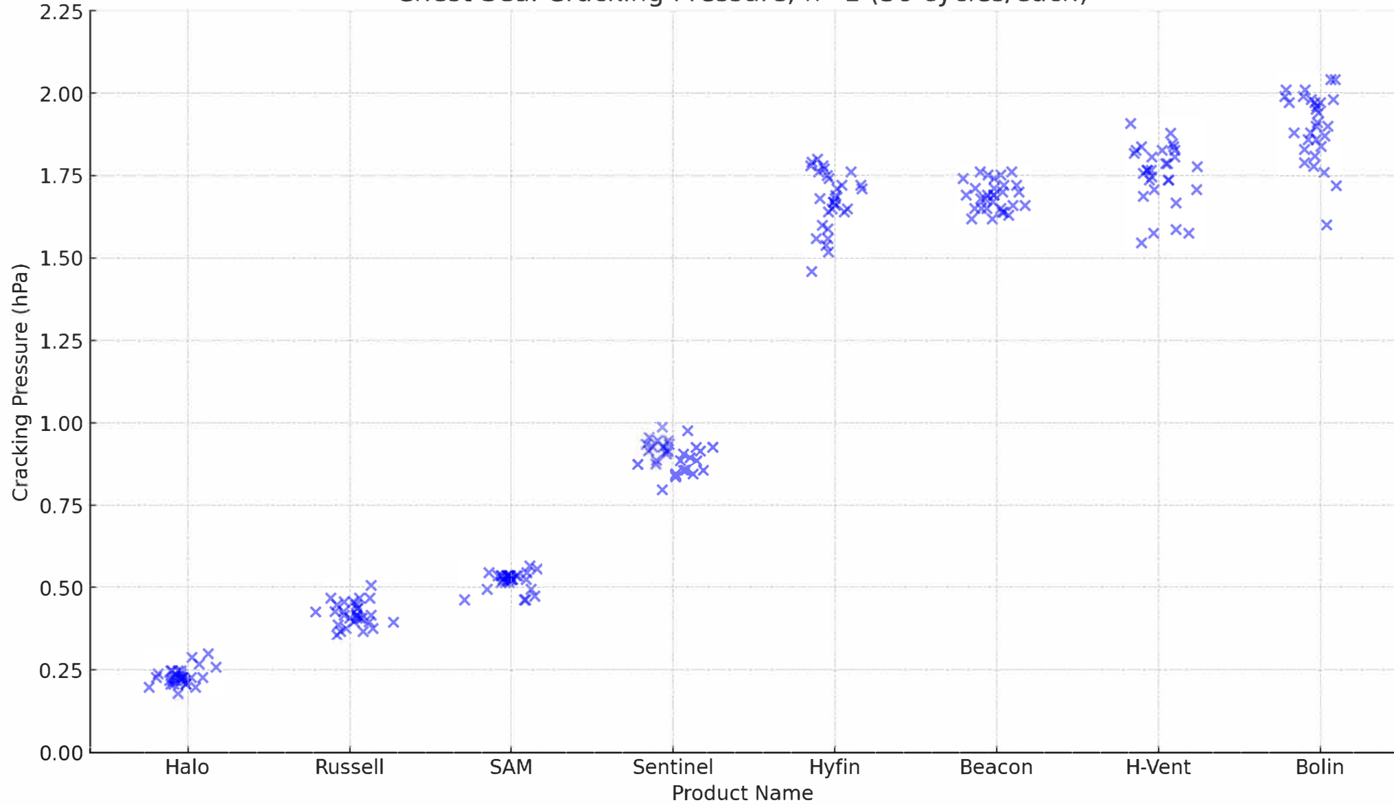
Chest Seal Cracking Pressure, n=1 (30 cycles/each)
